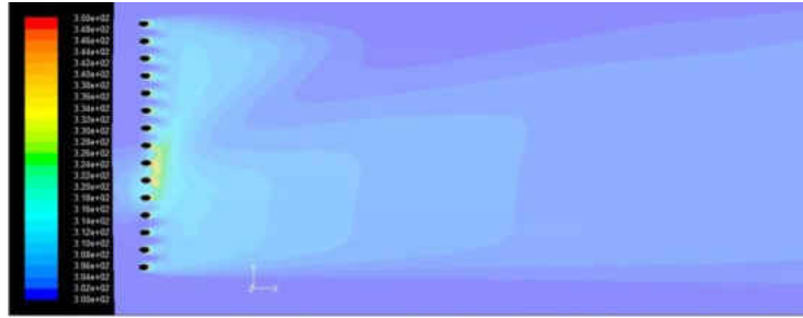
Figure 5.6: Temperature Contour of Case BR 1 Sr 0.1 at TS = 150, Spoke Location = 17.2°
