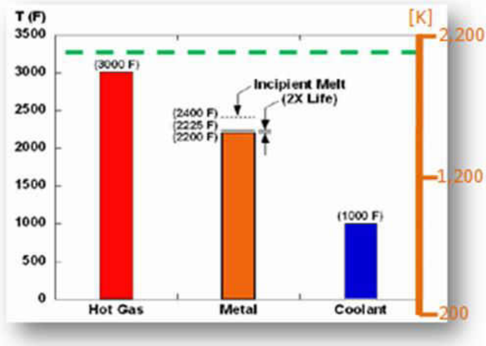
Figure 1.4: The Effect of Incipient Melting Temperature on Life Factor (N. D. Cardwell, 2005)
